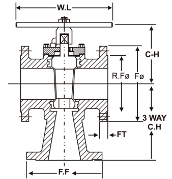
3-Way Valves
